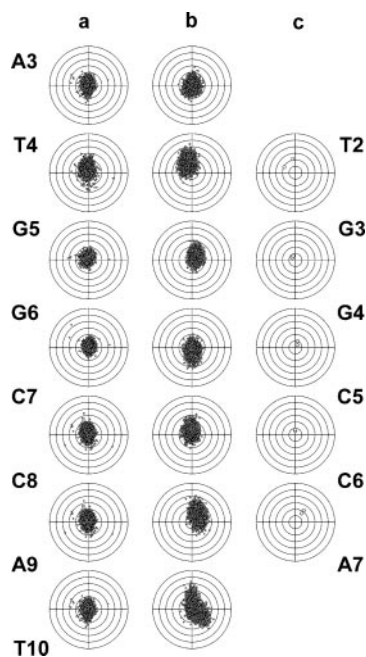
Fig. 4. Polar plots (“bending dials”) for all DNA internal steps in the d(GTATGGCCATAC) 2 oligonucleotide in the absence (a) and the presence (b) of two bonded trabectedin molecules. Two thousand individual points are for structures separated by 2 ps throughout the course of the last 4 ns of the MD trajectory. Viewed together, they constitute a probability density. Bending compressing the major groove is plotted on the northern hemisphere of the dial. For comparison, bending dials have also been calculated for the two independent (chromomycin) 2 -d(TTGGCCAA) 2 complexes found in the 1VAQ crystal structure (c). Coordinates for the covalent (trabectedin) 2 -d(GTATGGCCATAC) 2 complex have been deposited under Protein Data Bank code 2B01.
