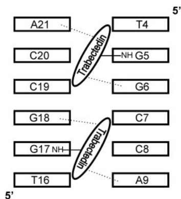
Fig. 2. Schematic representation of the central region of the oligonucleotide studied showing sequence composition and numbering. The covalent and hydrogen bonds (broken lines) between each trabectedin and the DNA are displayed.
