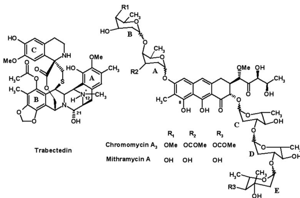
Fig. 1. Chemical structures of trabectedin (with three main subunits labeled A, B, and C) and aureolic acid derivatives, chromomycin A 3 and mithramycin A (with sugar rings labeled A-E). Atom positions relevant to the text have been numbered.
