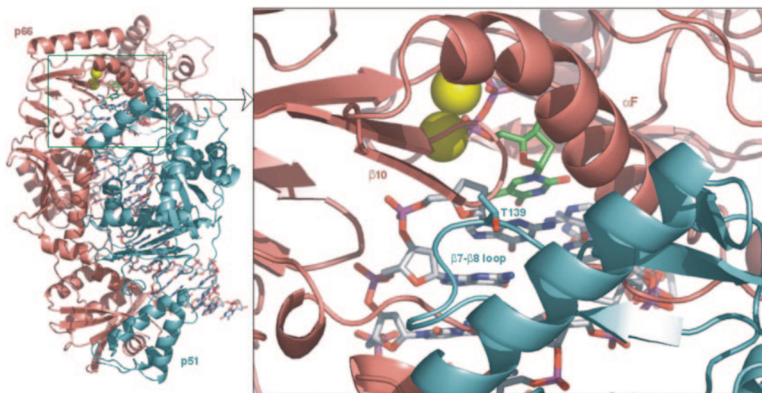
Fig. 1. Left, schematic representation of the dimeric structure of HIV-1 RT in complex with a DNA template:primer. The protein C\alpha trace of each subunit is shown as a ribbon colored pink for p66 and cyan for p51, whereas the DNA molecule (C atoms in gray) and the incoming deoxythymidine triphosphate nucleotide (C atoms in green) are displayed as sticks. The Mg^{2+} ions at the active site are shown as yellow spheres. Right, enlarged view of the framed area shown on the left providing detail of the location of the \beta 7 - \beta 8 loop of p51 at the subunit interface which includes Thr139 (side chain as sticks with C atoms in cyan and the OH oxygen in red).
