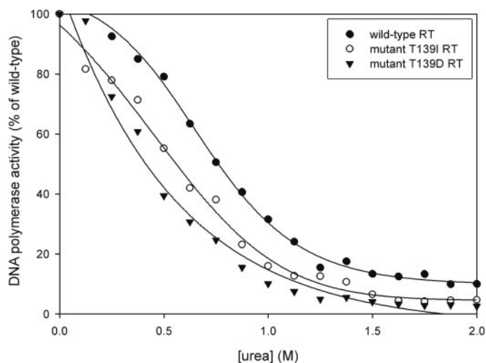
Fig. 4. Effect of urea on the catalytic activity of mutant T139I, T139D, and wild-type HIV-1 RTs.
