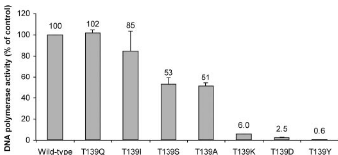
Fig. 2. Catalytic RNA-dependent DNA polymerase activity of mutant T139Q, T139I, T139S, T139A, T139K, T139D, and T139Y HIV-1 RT enzymes. 8 ng of wild type, 11 ng of T139A, 6 ng of T139Q, 61 ng of T139Y, 575 ng of T139K, 6 ng of T139I, 9 ng of T139S, and 137 ng of T139D mutant enzyme (protein) were used in the enzyme assays. Data ( \pm S.D.) are the means of at least two to three independent experiments.
