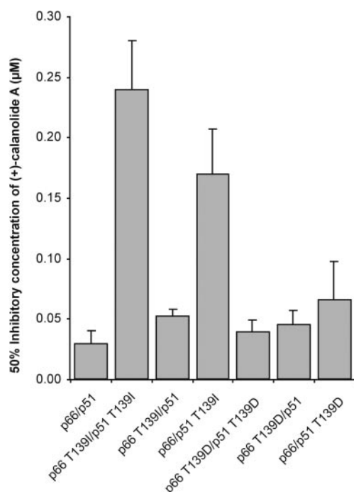
Fig. 3. Inhibitory activity of (+)-calanolide A against the catalytic activity of wild-type and mutant HIV-1 RT enzymes that contain the T139I or T139D mutation solely in the p66, solely in the p51, or both in the p66 and p51 subunits.
